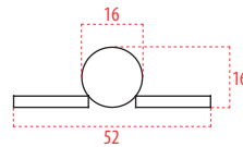
90° Dönüş Rayı 90° Turning Track (radius curved)
